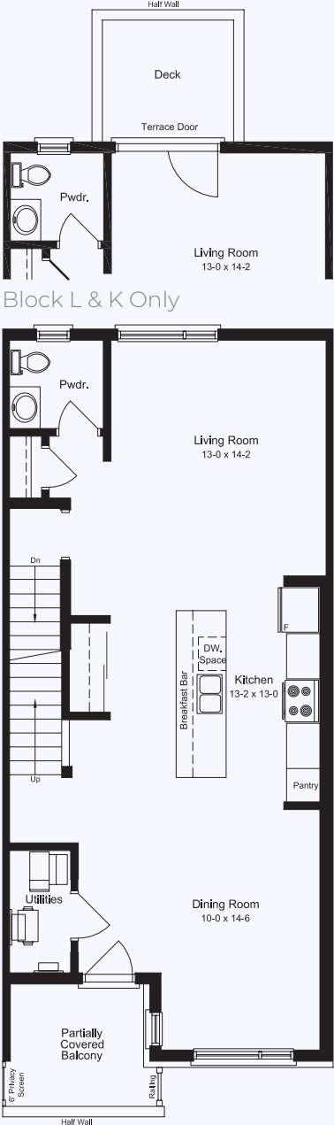
SECOND FLOOR 830 Sq.Ft.
