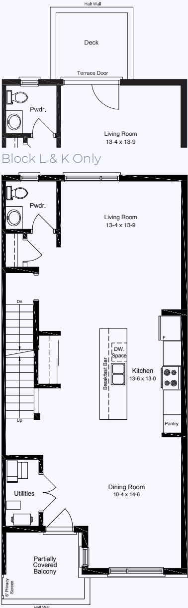
SECOND FLOOR 852 Sq.Ft.
