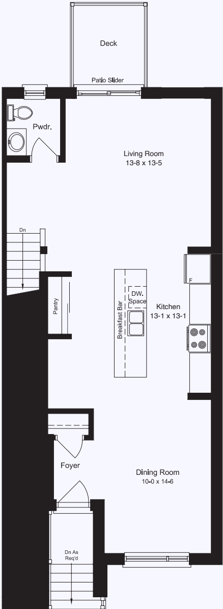
MAIN FLOOR 778 Sq.Ft.
